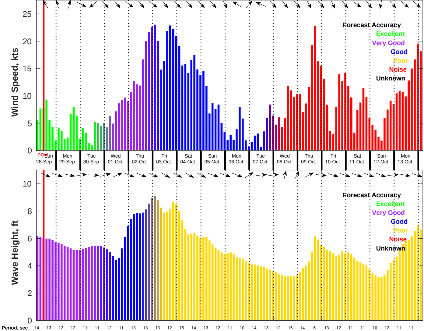
Wind & Wave Forecast for NDBC 46011 from 28-Sep-2025 04:00:00 to 14-Oct-2025 04:00:00
