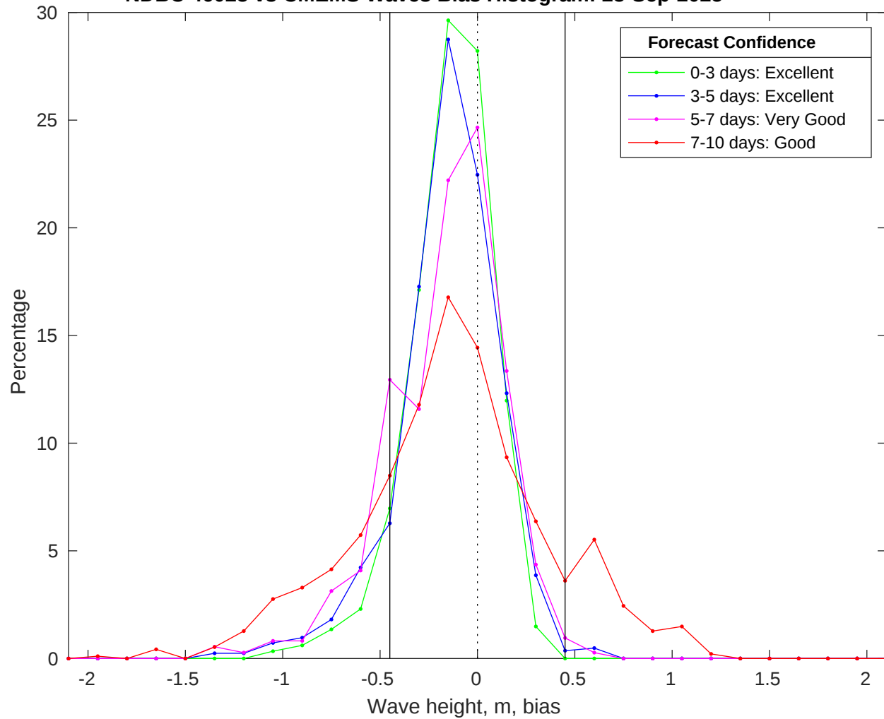
NDBC 46028 vs CMEMS Waves Bias Histogram: 28-Sep-2025
