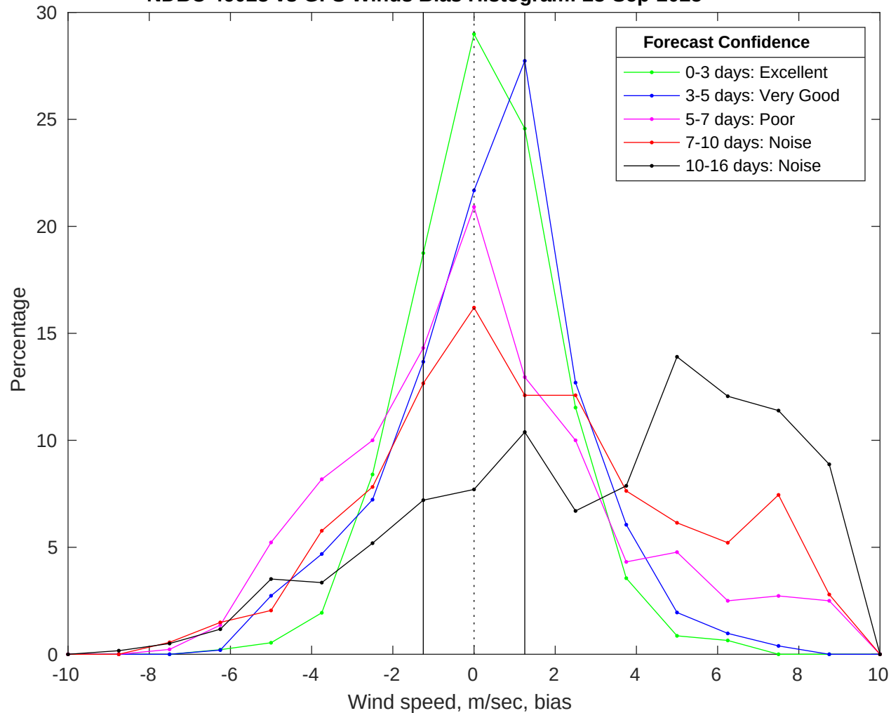
NDBC 46028 vs GFS Winds Bias Histogram: 28-Sep-2025
