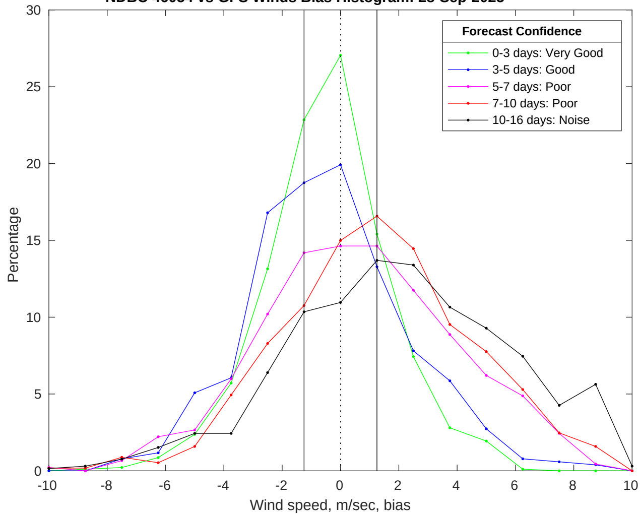
NDBC 46054 vs GFS Winds Bias Histogram: 28-Sep-2025
