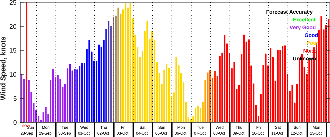
GFS Wind Speed Forecast for NDBC 46054 from 28-Sep-2025 04:00:00 to 14-Oct-2025 04:00:00
