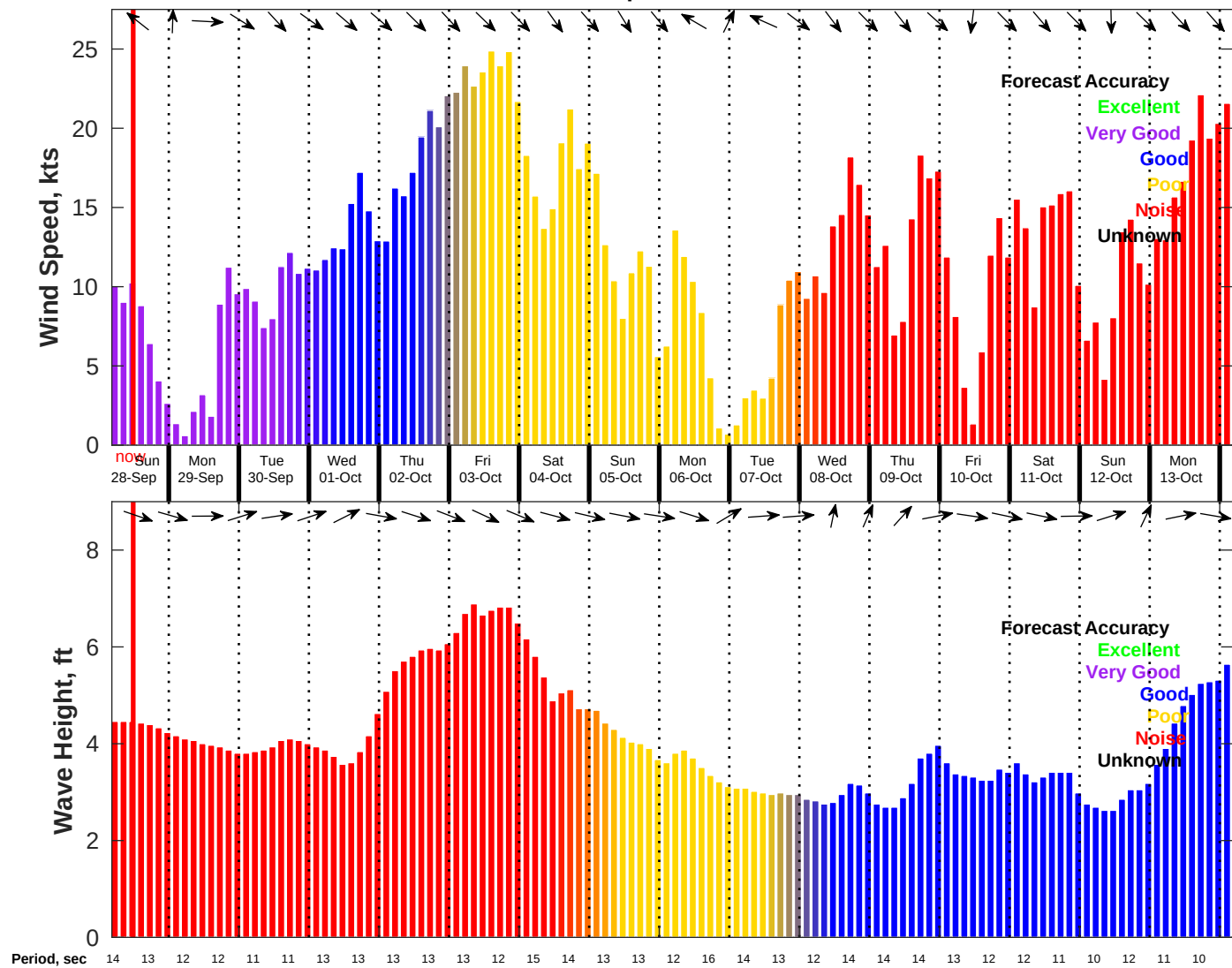
Wind & Wave Forecast for NDBC 46054 from 28-Sep-2025 04:00:00 to 14-Oct-2025 04:00:00
