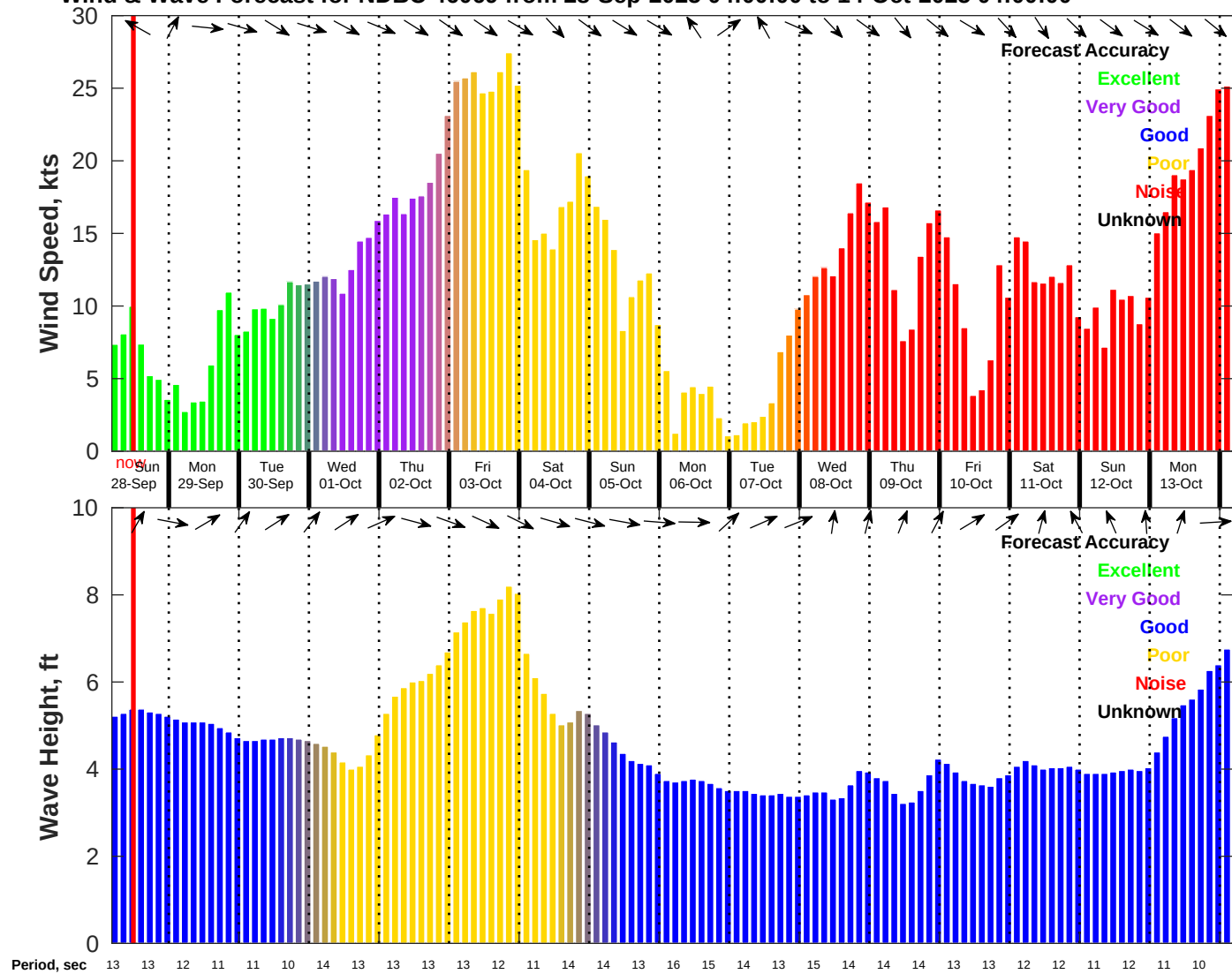
Wind & Wave Forecast for NDBC 46069 from 28-Sep-2025 04:00:00 to 14-Oct-2025 04:00:00
