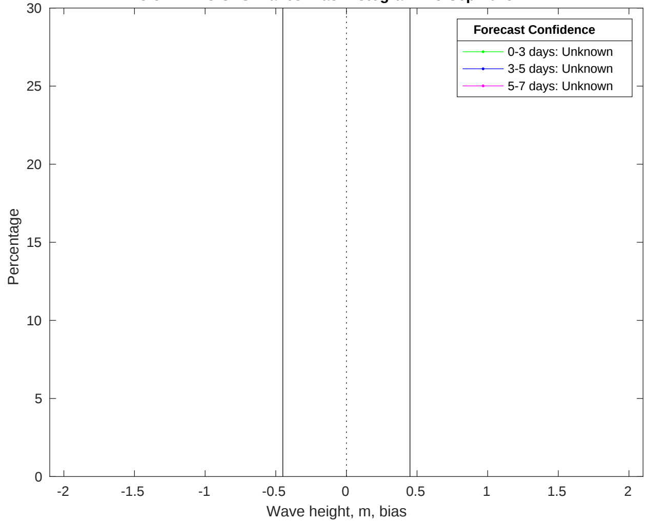
NDBC 51211 vs GFS Waves Bias Histogram: 28-Sep-2025
