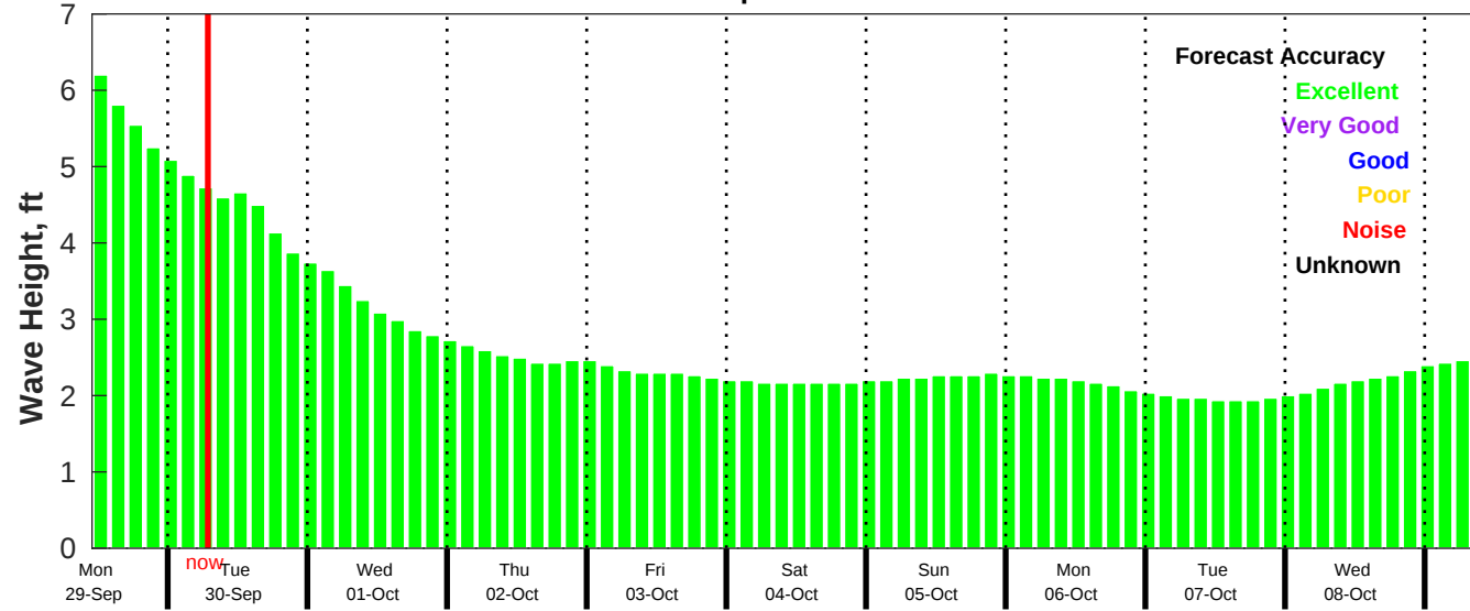
CMEMS Wave Forecast for NDBC 52211 from 28-Sep-2025 11:00:00 to 08-Oct-2025 11:00:00
