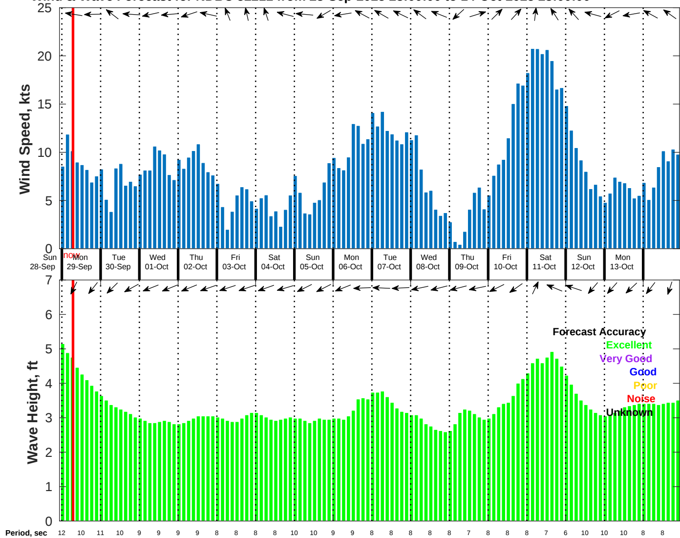
Wind & Wave Forecast for NDBC 52211 from 28-Sep-2025 23:00:00 to 14-Oct-2025 23:00:00
