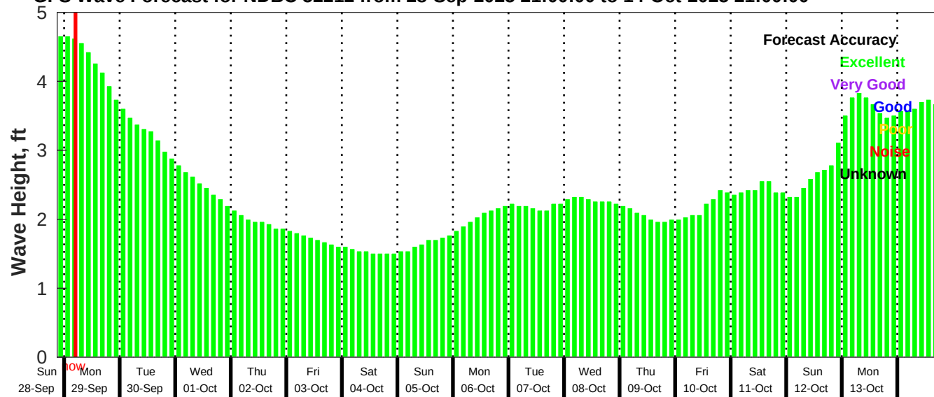
GFS Wave Forecast for NDBC 52212 from 28-Sep-2025 21:00:00 to 14-Oct-2025 21:00:00
