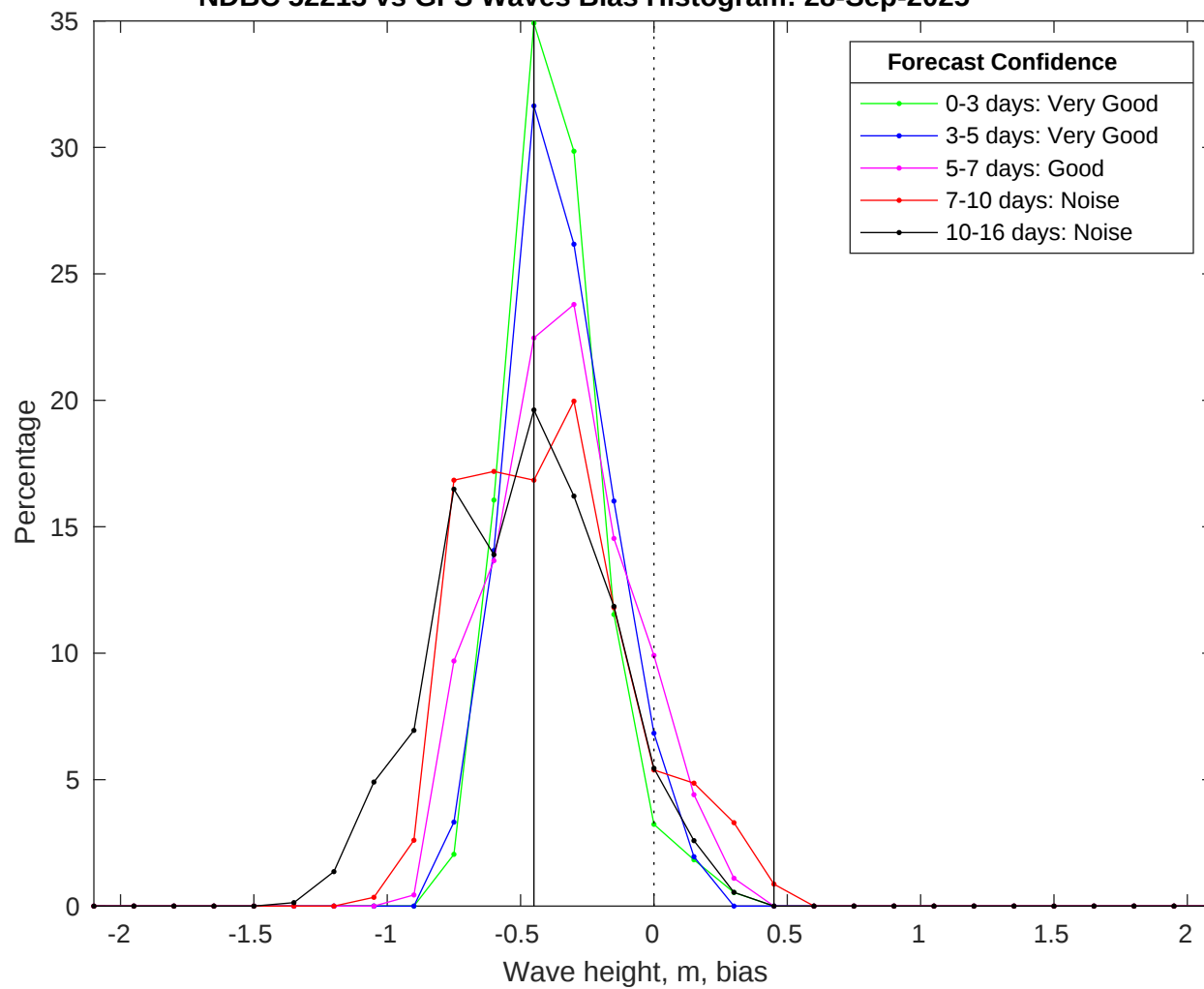
NDBC 52213 vs GFS Waves Bias Histogram: 28-Sep-2025
