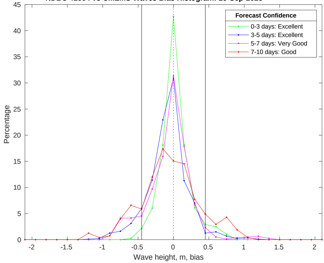
NDBC 41004 vs CMEMS Waves Bias Histogram: 29-Sep-2025
