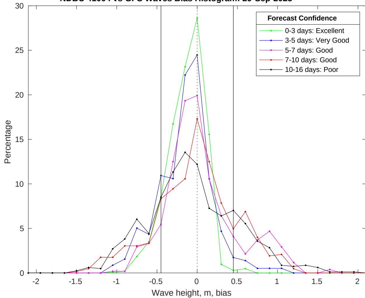
NDBC 41004 vs GFS Waves Bias Histogram: 29-Sep-2025
