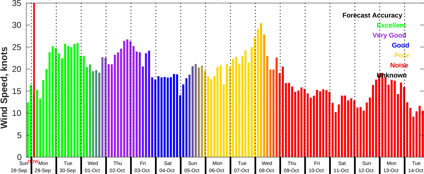
GFS Wind Speed Forecast for NDBC 41004 from 28-Sep-2025 19:00:00 to 14-Oct-2025 19:00:00
