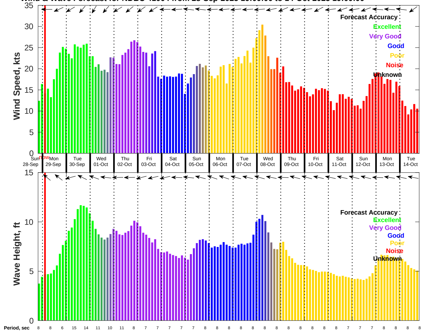
Wind & Wave Forecast for NDBC 41004 from 28-Sep-2025 19:00:00 to 14-Oct-2025 19:00:00
