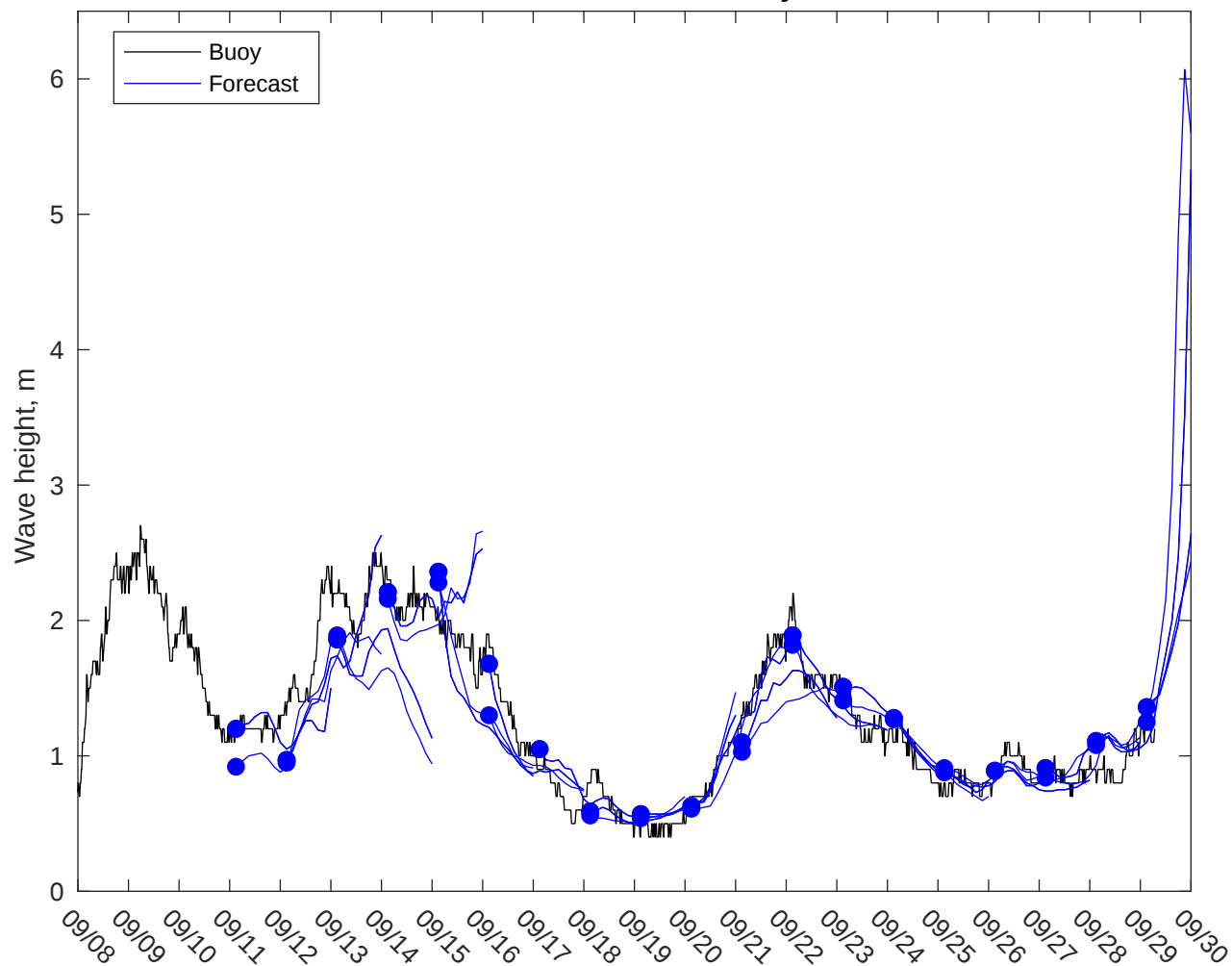
NDBC 41013 vs CMEMS Waves: 3 to 5 day forecast
