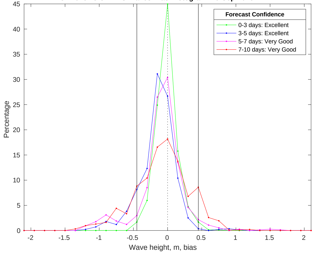
NDBC 41013 vs CMEMS Waves Bias Histogram: 29-Sep-2025
