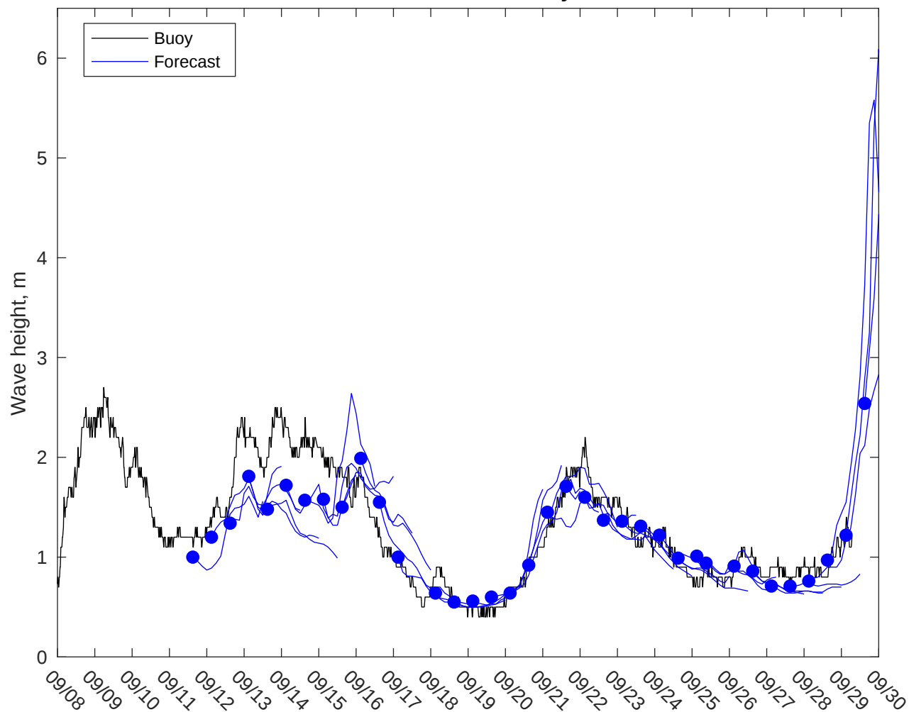
NDBC 41013 vs GFS Waves: 3 to 5 day forecast
