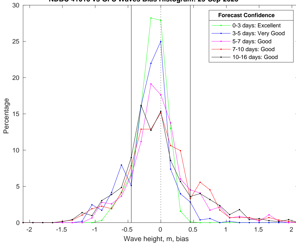
NDBC 41013 vs GFS Waves Bias Histogram: 29-Sep-2025
