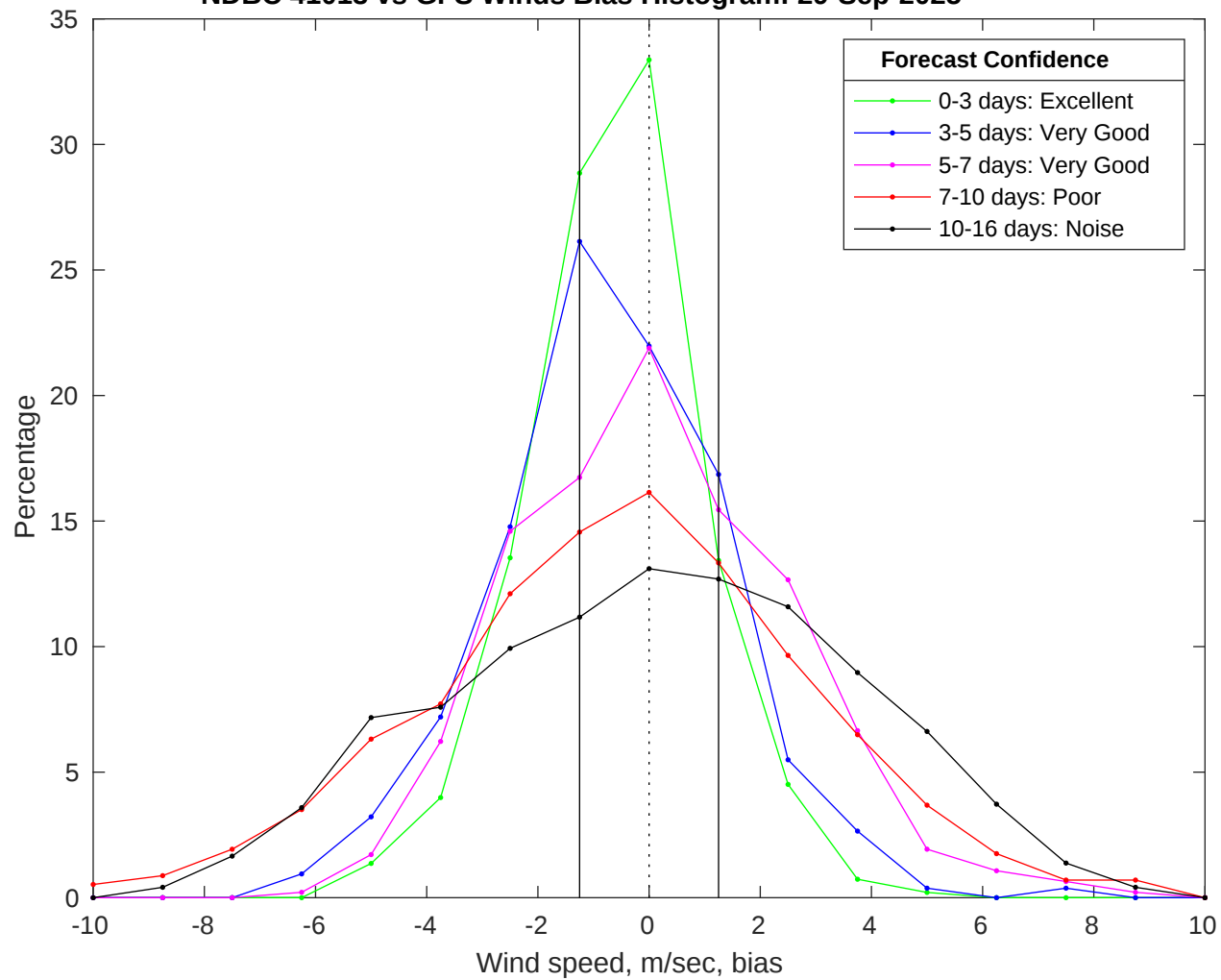
NDBC 41013 vs GFS Winds Bias Histogram: 29-Sep-2025
