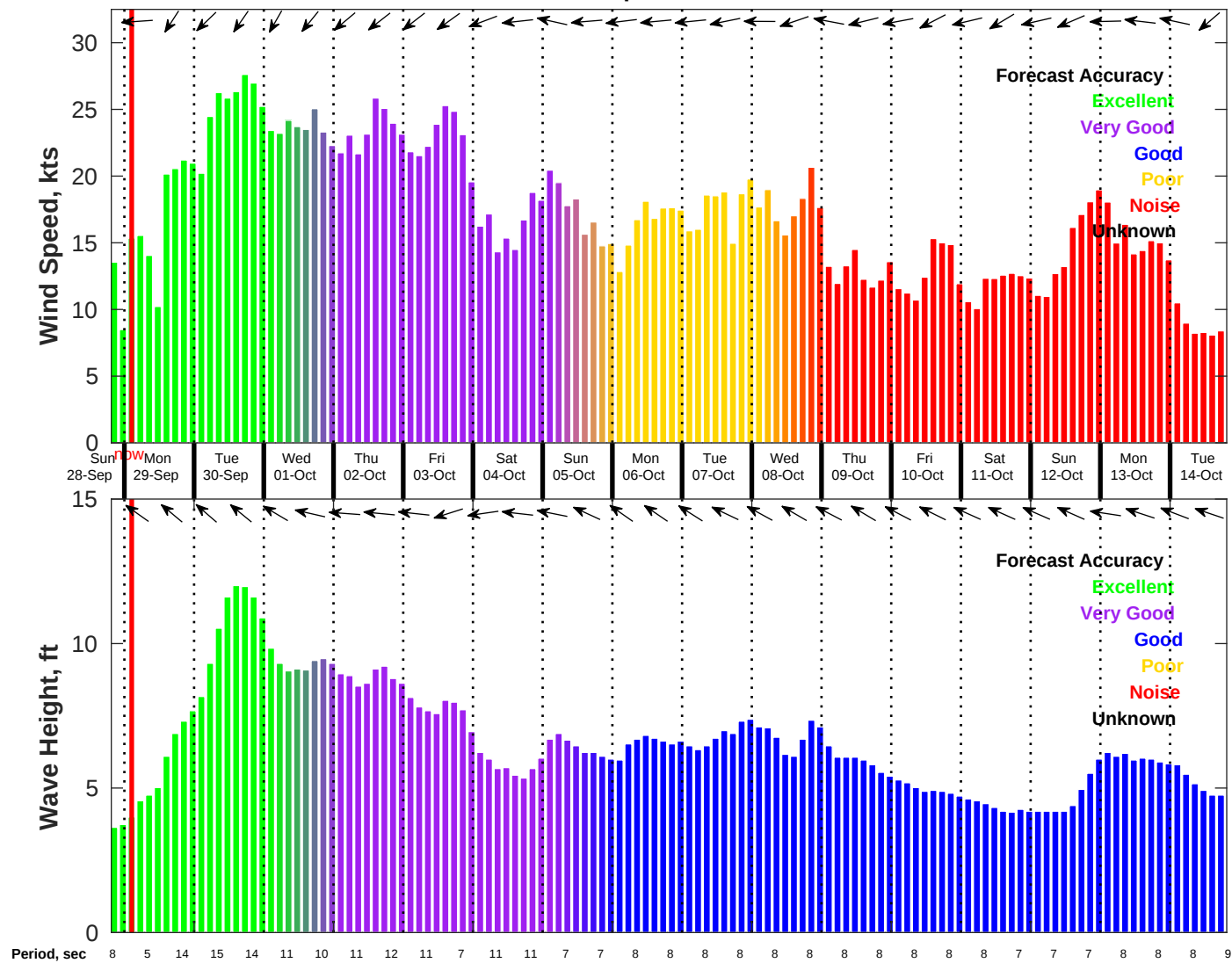
Wind & Wave Forecast for NDBC 41013 from 28-Sep-2025 19:00:00 to 14-Oct-2025 19:00:00
