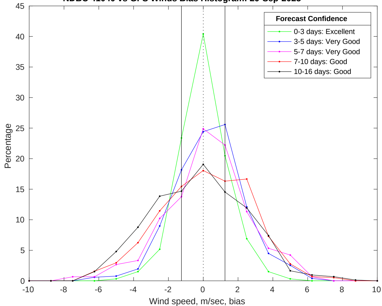
NDBC 41040 vs GFS Winds Bias Histogram: 29-Sep-2025
