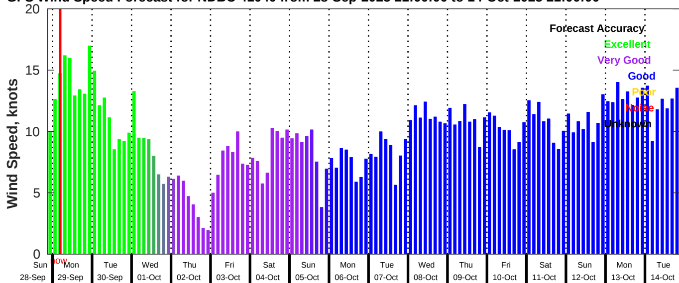
GFS Wind Speed Forecast for NDBC 41040 from 28-Sep-2025 21:00:00 to 14-Oct-2025 21:00:00
