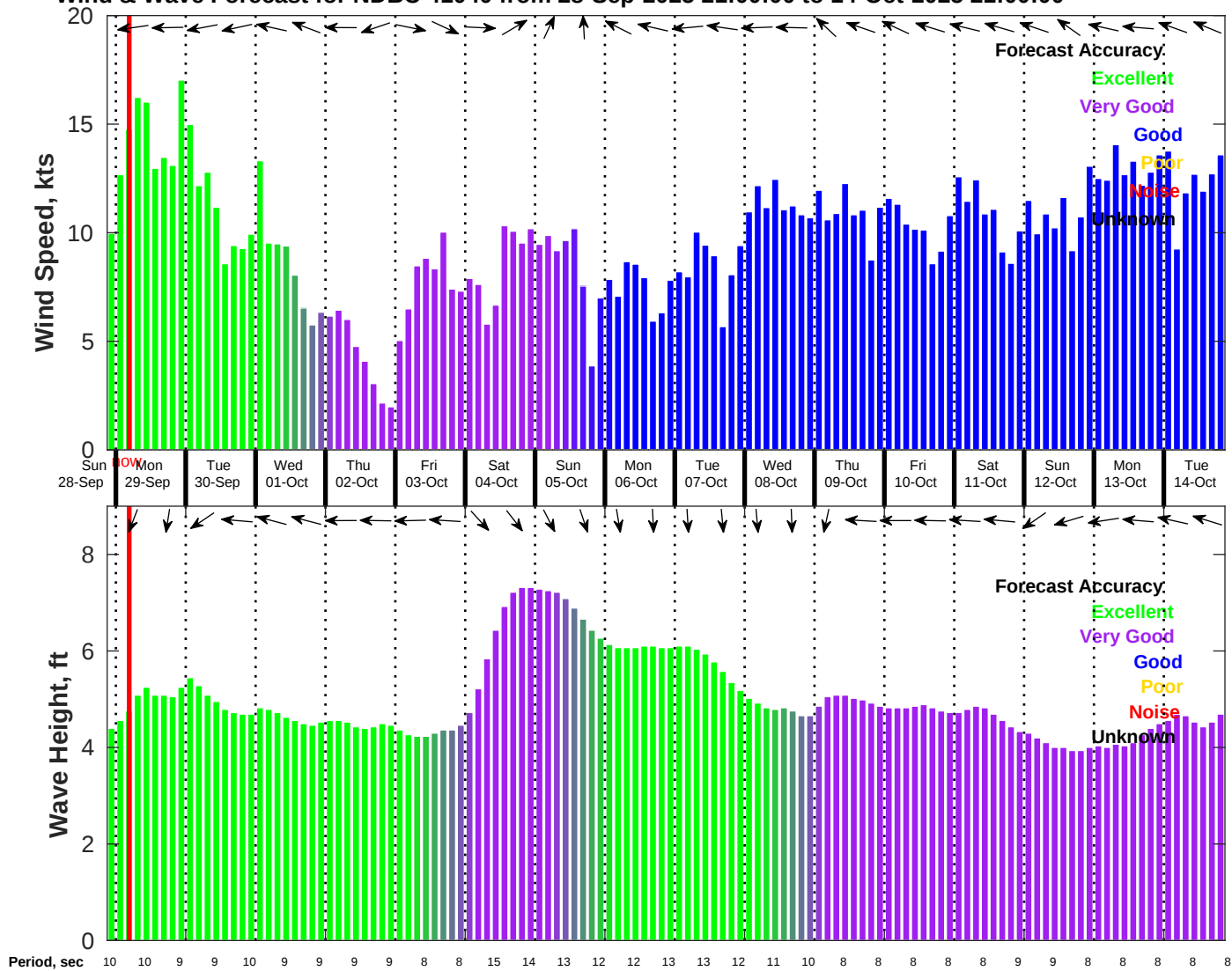
Wind & Wave Forecast for NDBC 41040 from 28-Sep-2025 21:00:00 to 14-Oct-2025 21:00:00
