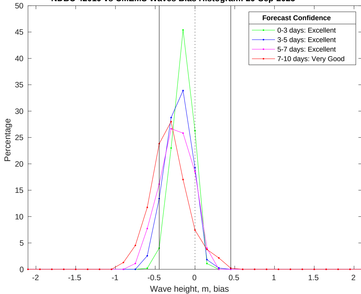
NDBC 42019 vs CMEMS Waves Bias Histogram: 29-Sep-2025
