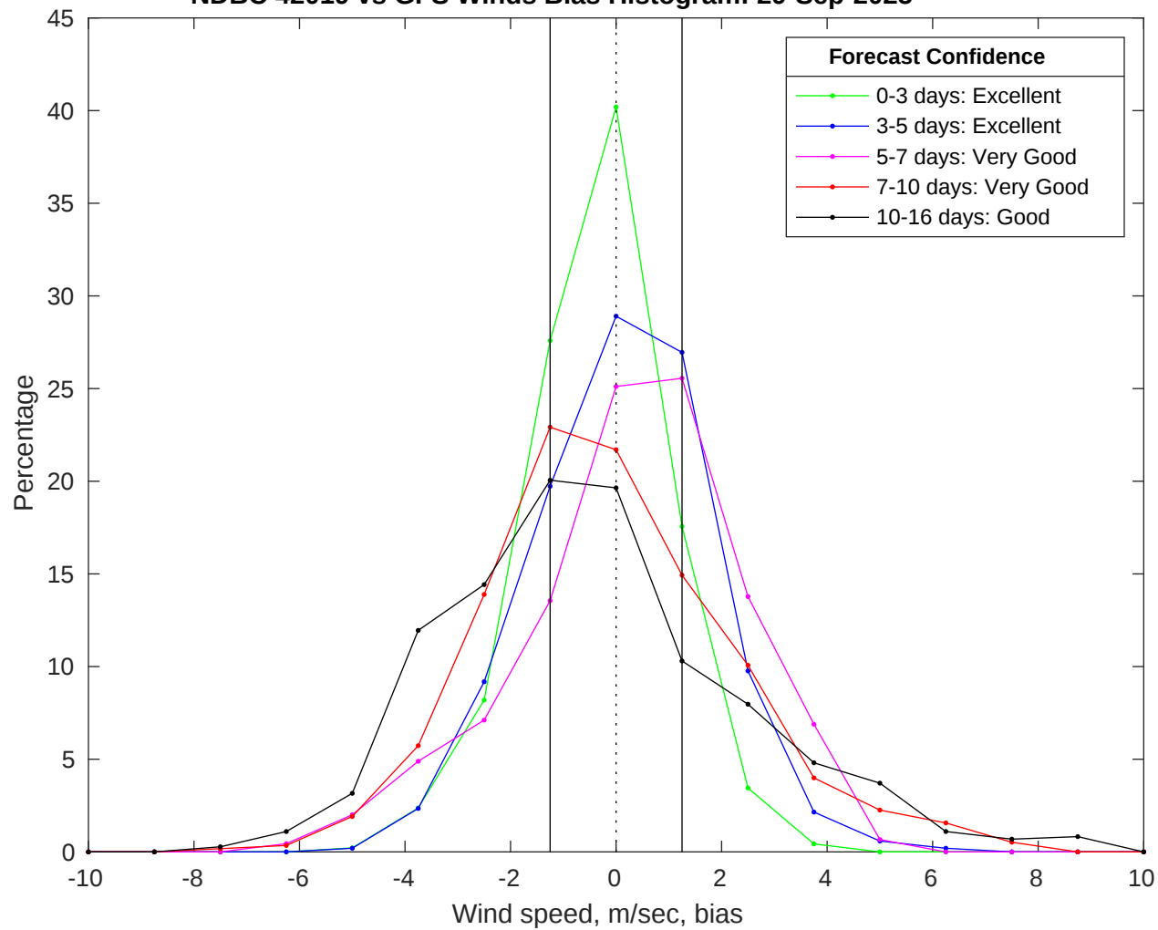
NDBC 42019 vs GFS Winds Bias Histogram: 29-Sep-2025
