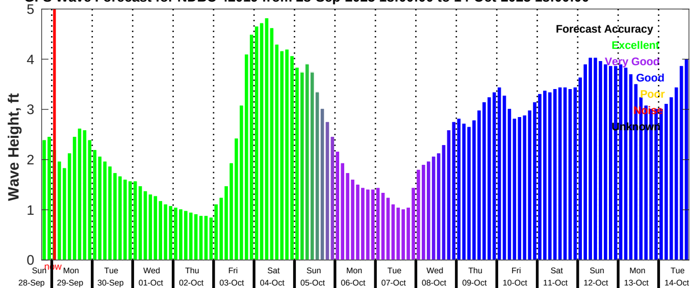
GFS Wave Forecast for NDBC 42019 from 28-Sep-2025 18:00:00 to 14-Oct-2025 18:00:00
