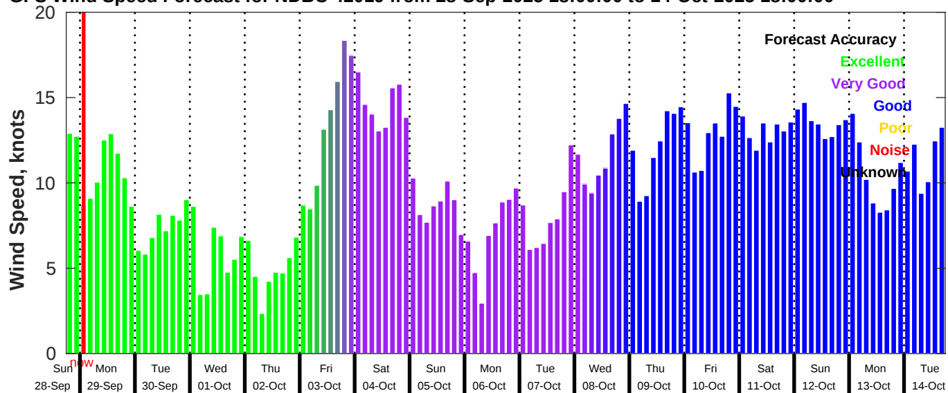
GFS Wind Speed Forecast for NDBC 42019 from 28-Sep-2025 18:00:00 to 14-Oct-2025 18:00:00
