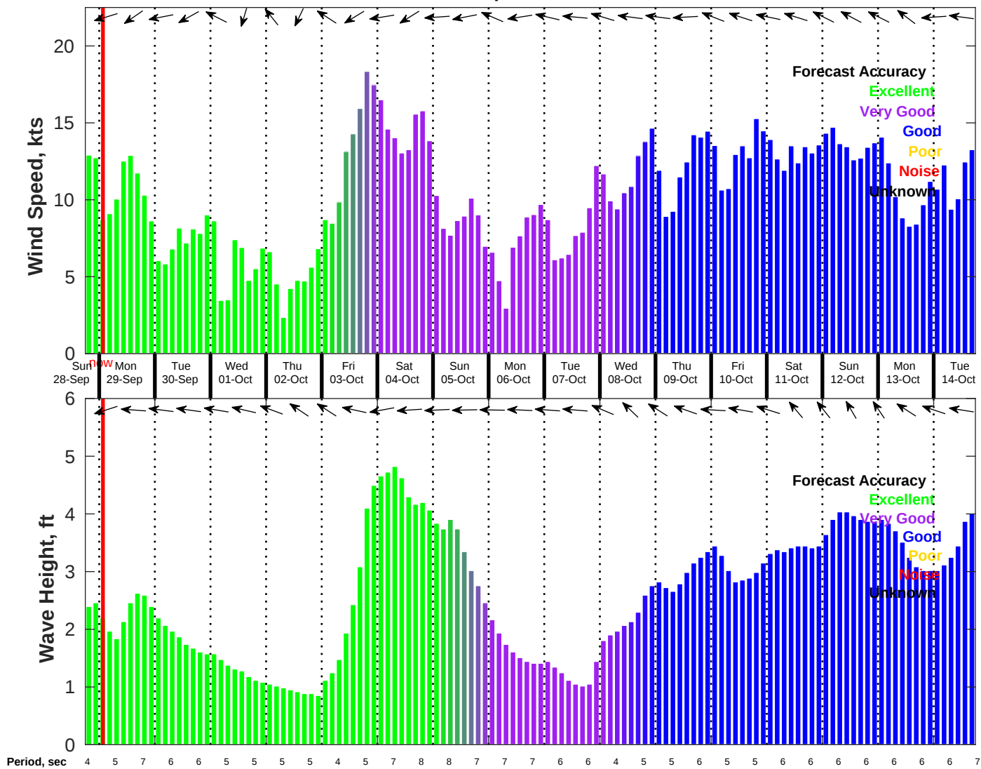
Wind & Wave Forecast for NDBC 42019 from 28-Sep-2025 18:00:00 to 14-Oct-2025 18:00:00
