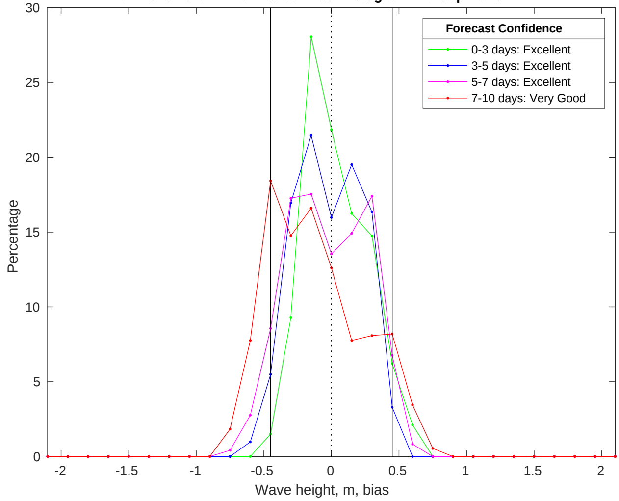
NDBC 42020 vs CMEMS Waves Bias Histogram: 29-Sep-2025
