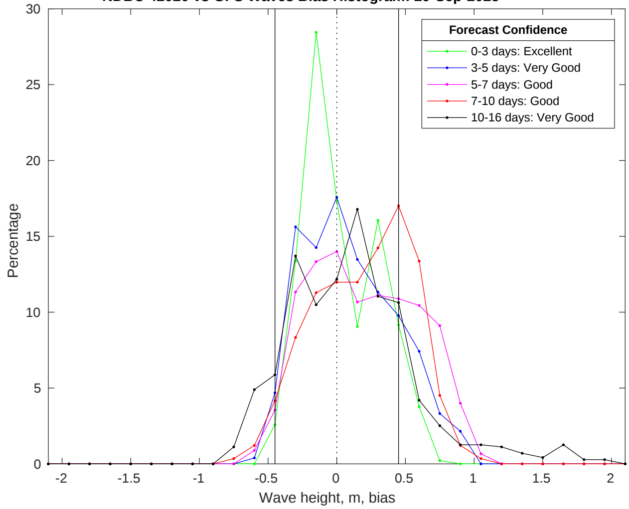
NDBC 42020 vs GFS Waves Bias Histogram: 29-Sep-2025
