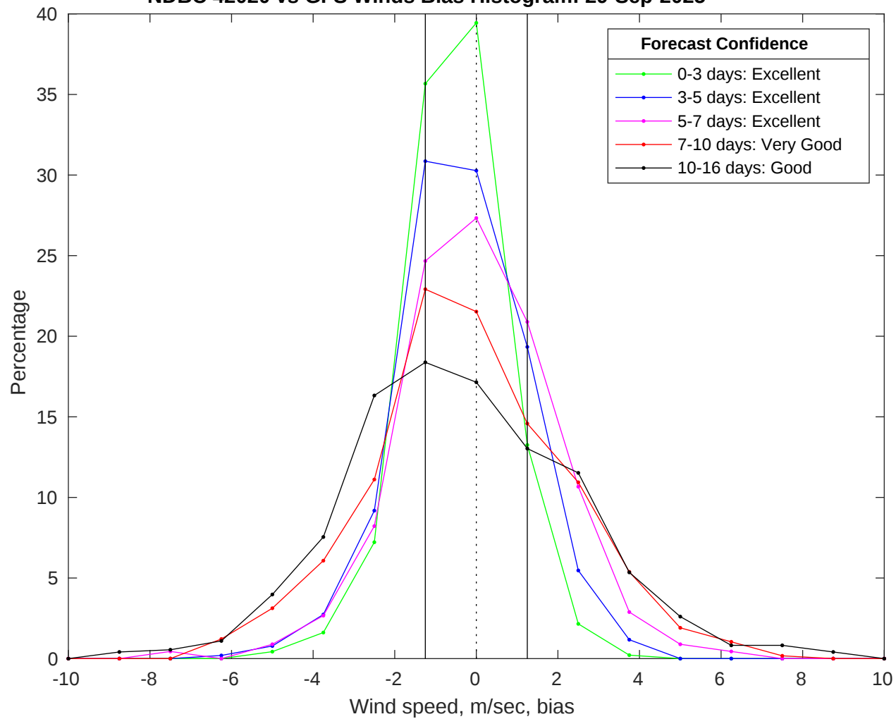
NDBC 42020 vs GFS Winds Bias Histogram: 29-Sep-2025
