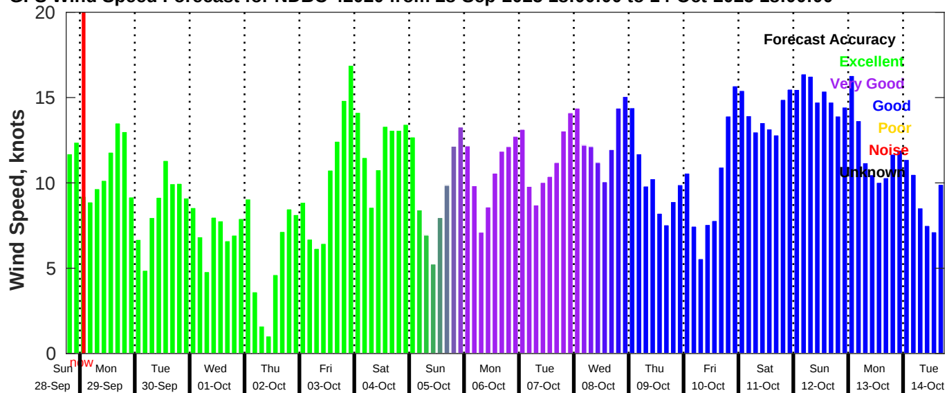
GFS Wind Speed Forecast for NDBC 42020 from 28-Sep-2025 18:00:00 to 14-Oct-2025 18:00:00
