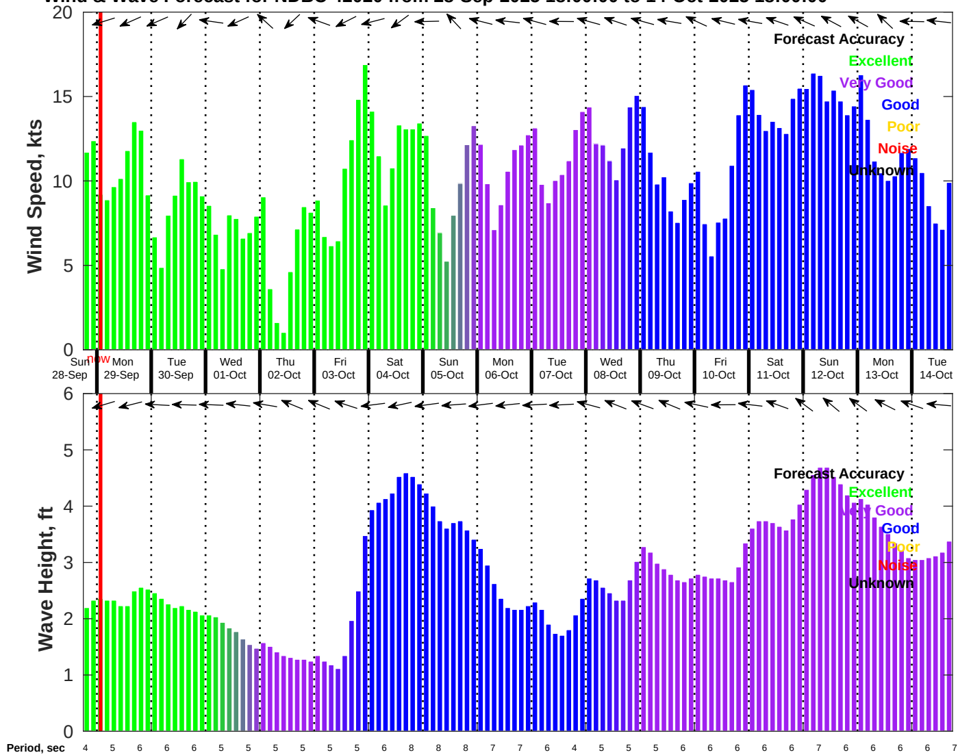
Wind & Wave Forecast for NDBC 42020 from 28-Sep-2025 18:00:00 to 14-Oct-2025 18:00:00
