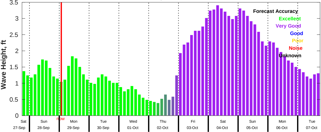
CMEMS Wave Forecast for NDBC 42035 from 27-Sep-2025 18:00:00 to 07-Oct-2025 18:00:00
