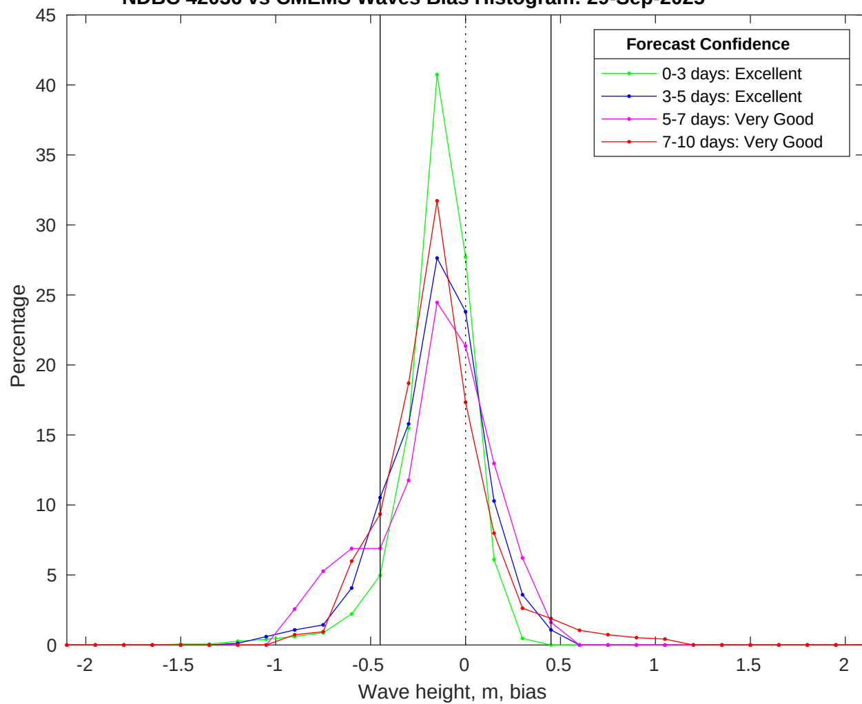
NDBC 42036 vs CMEMS Waves Bias Histogram: 29-Sep-2025
