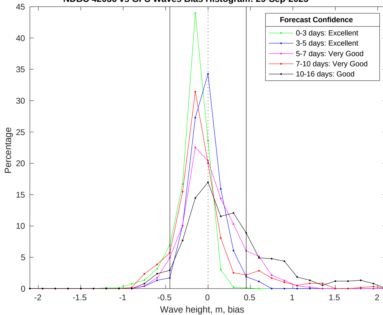
NDBC 42036 vs GFS Waves Bias Histogram: 29-Sep-2025
