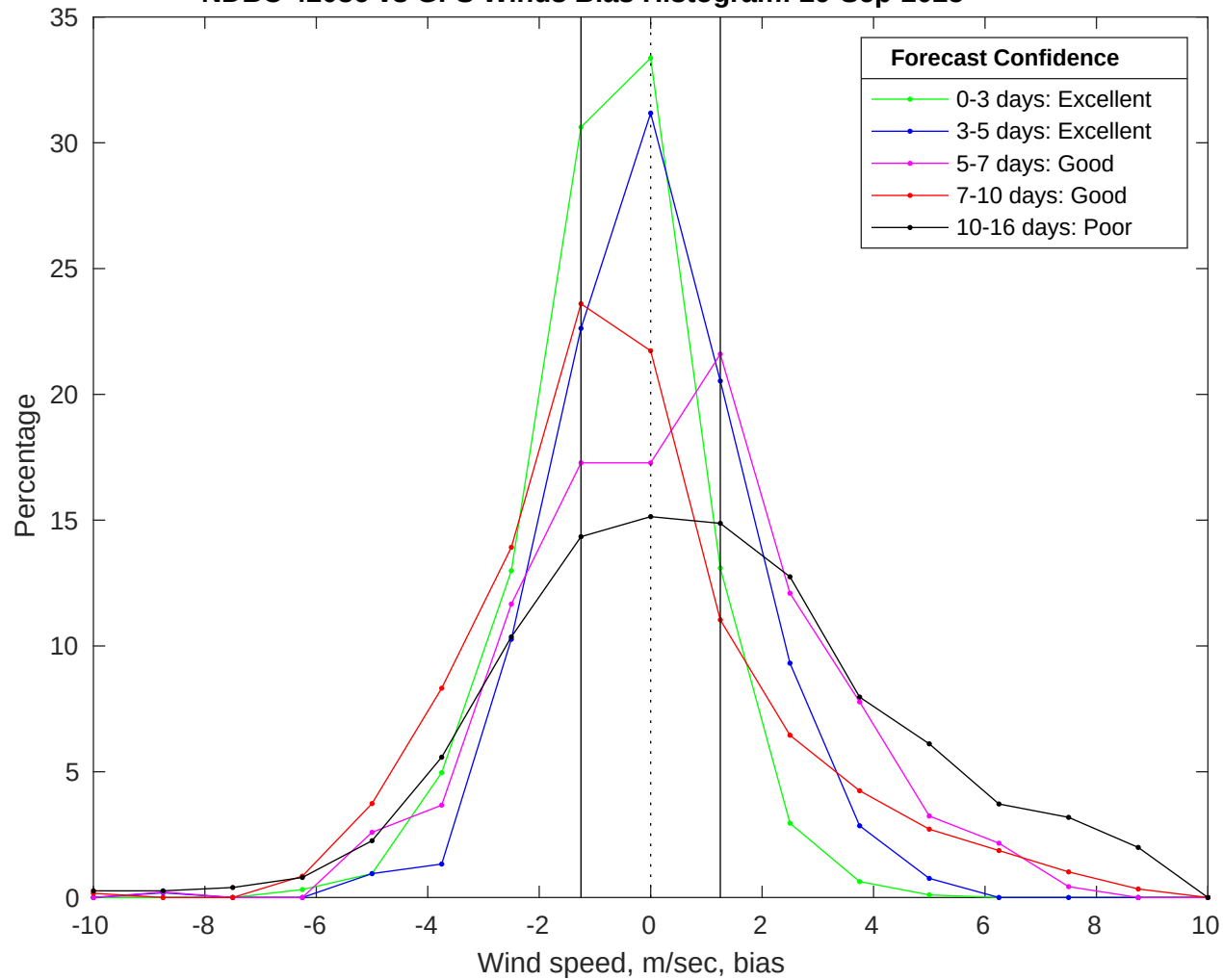
NDBC 42036 vs GFS Winds Bias Histogram: 29-Sep-2025
