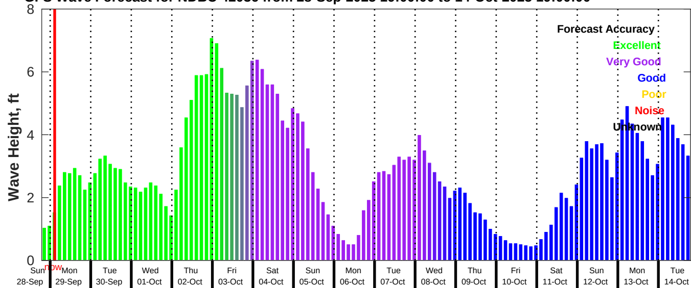
GFS Wave Forecast for NDBC 42036 from 28-Sep-2025 19:00:00 to 14-Oct-2025 19:00:00
