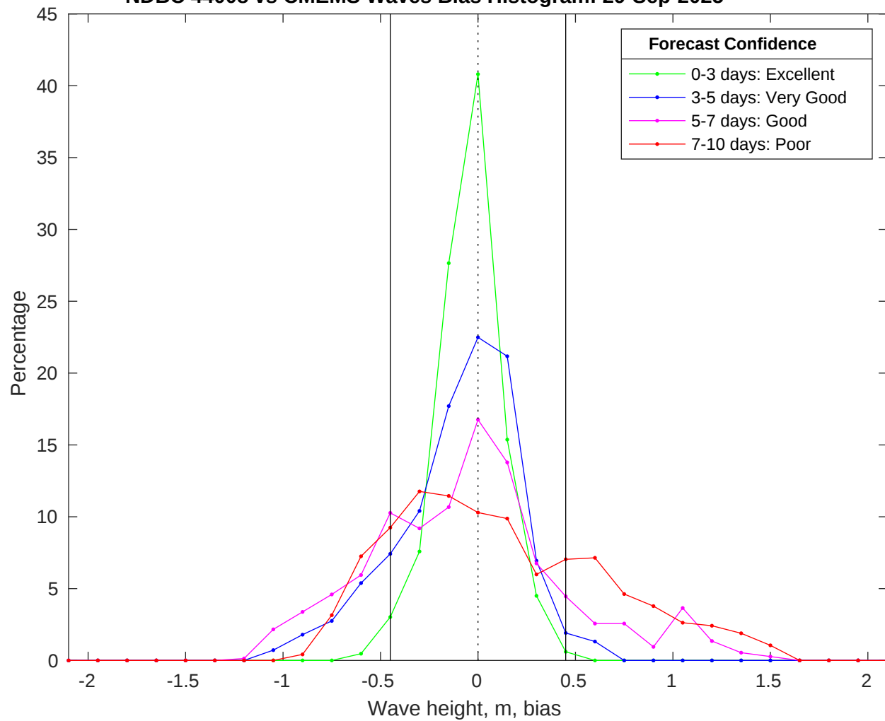
NDBC 44008 vs CMEMS Waves Bias Histogram: 29-Sep-2025
