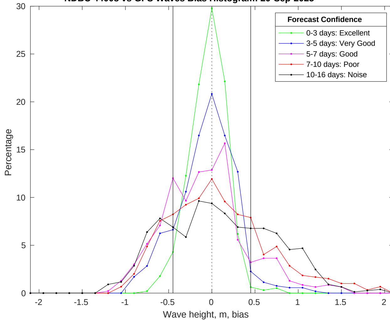
NDBC 44008 vs GFS Waves Bias Histogram: 29-Sep-2025
