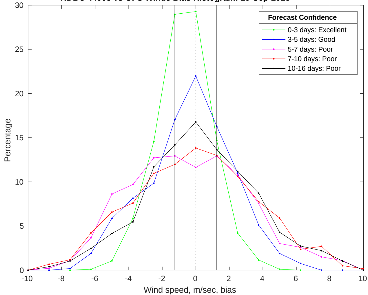
NDBC 44008 vs GFS Winds Bias Histogram: 29-Sep-2025
