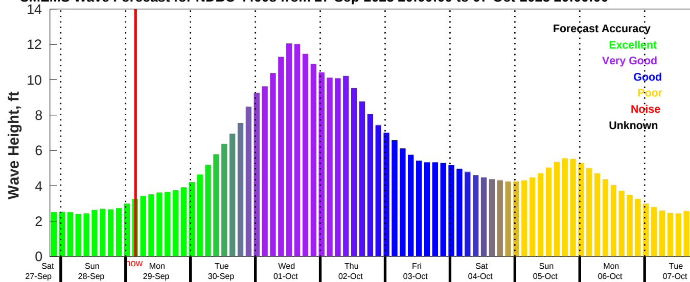
CMEMS Wave Forecast for NDBC 44008 from 27-Sep-2025 20:00:00 to 07-Oct-2025 20:00:00
