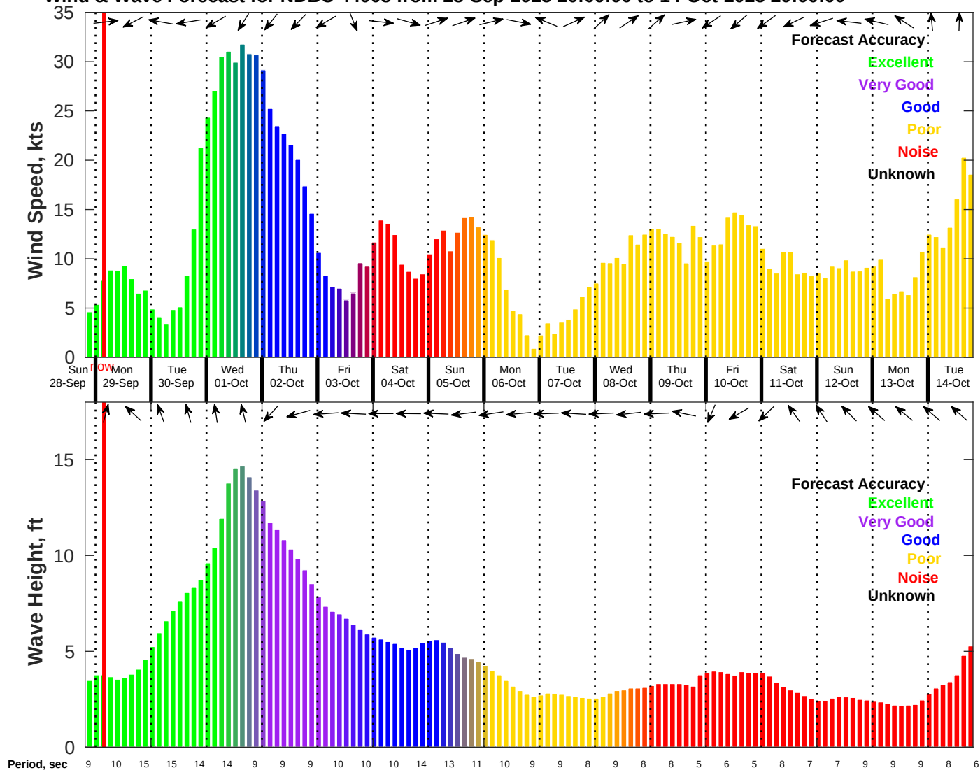
Wind & Wave Forecast for NDBC 44008 from 28-Sep-2025 20:00:00 to 14-Oct-2025 20:00:00
