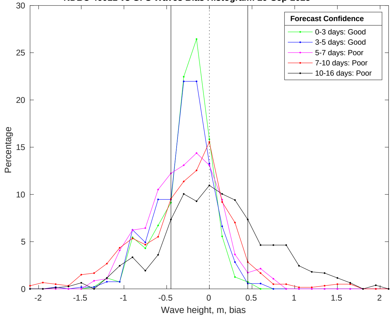
NDBC 46011 vs GFS Waves Bias Histogram: 29-Sep-2025
