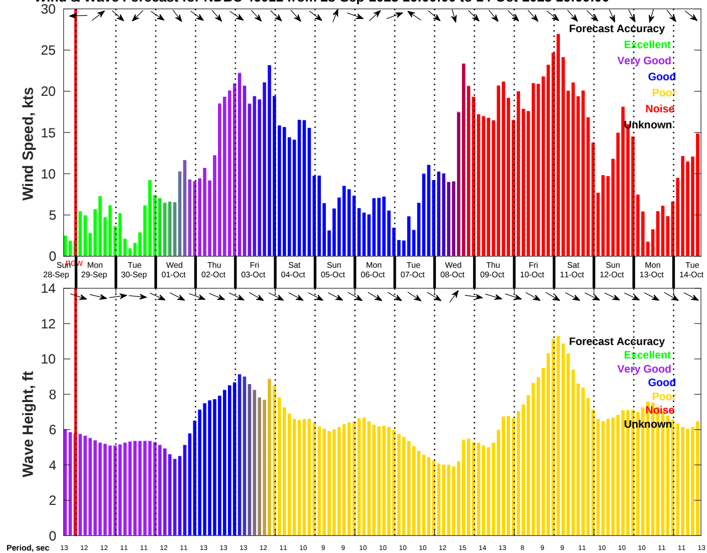
Wind & Wave Forecast for NDBC 46011 from 28-Sep-2025 16:00:00 to 14-Oct-2025 16:00:00
