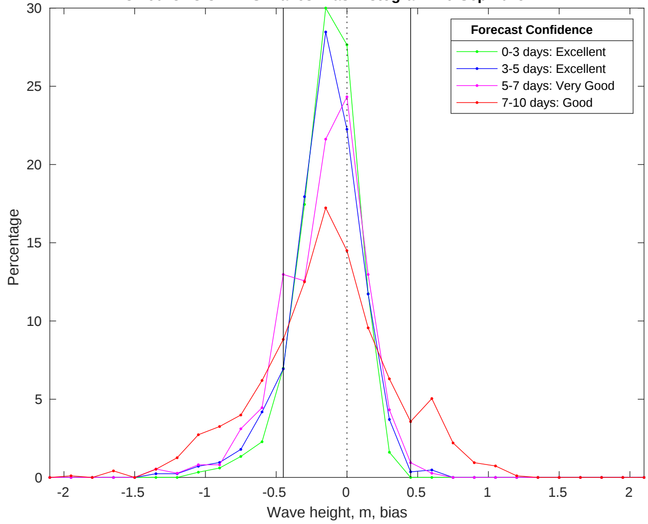
NDBC 46028 vs CMEMS Waves Bias Histogram: 29-Sep-2025
