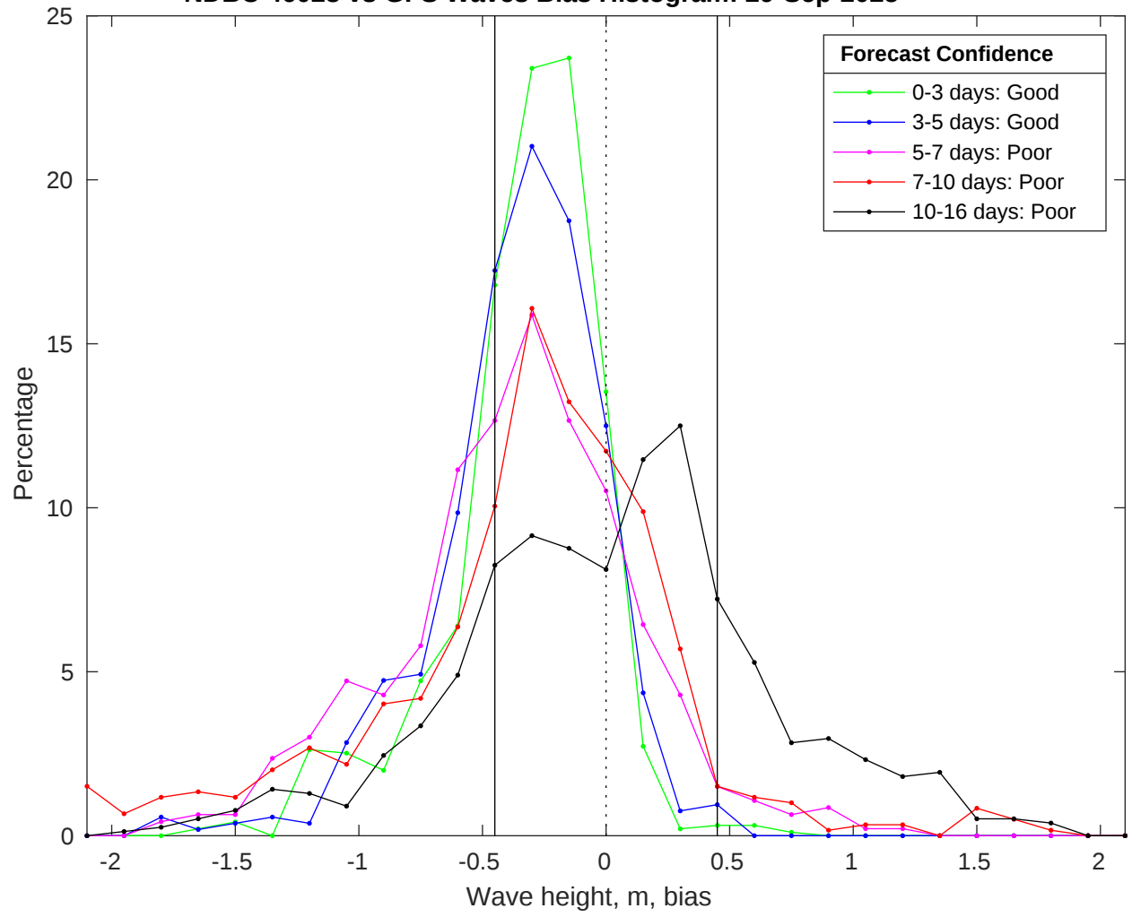
NDBC 46028 vs GFS Waves Bias Histogram: 29-Sep-2025
