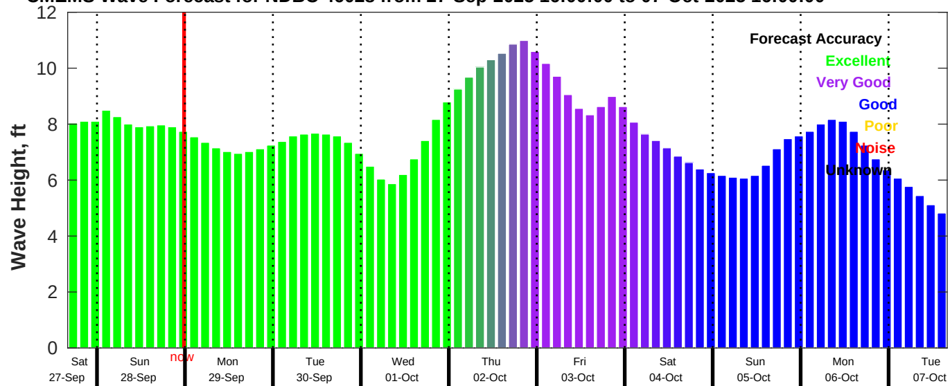
CMEMS Wave Forecast for NDBC 46028 from 27-Sep-2025 16:00:00 to 07-Oct-2025 16:00:00
